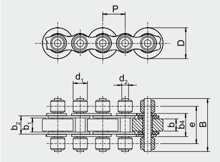
Design OS without of washers
