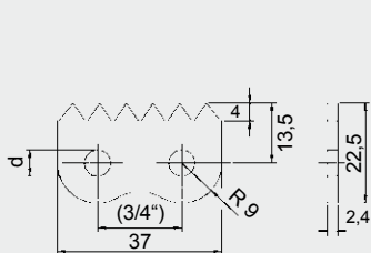
For chain M 128 A SL: Design 103.64
