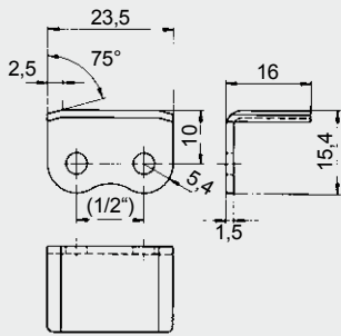
For chain L 85 SL: Design 203.8
