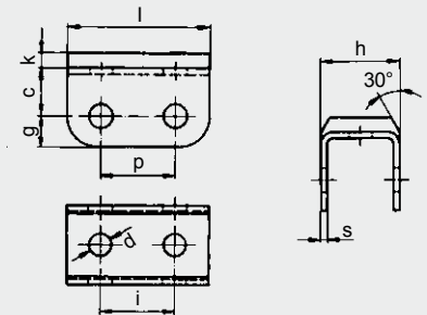
Design 303.9 with rubber cover
