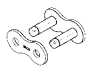
Outer link Standard designation A
