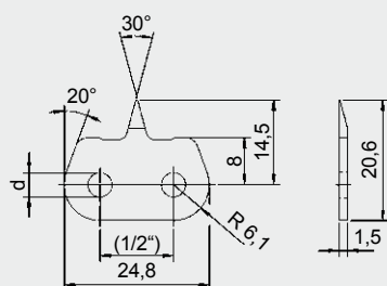
For chain L 85 SL: Design 112.09
